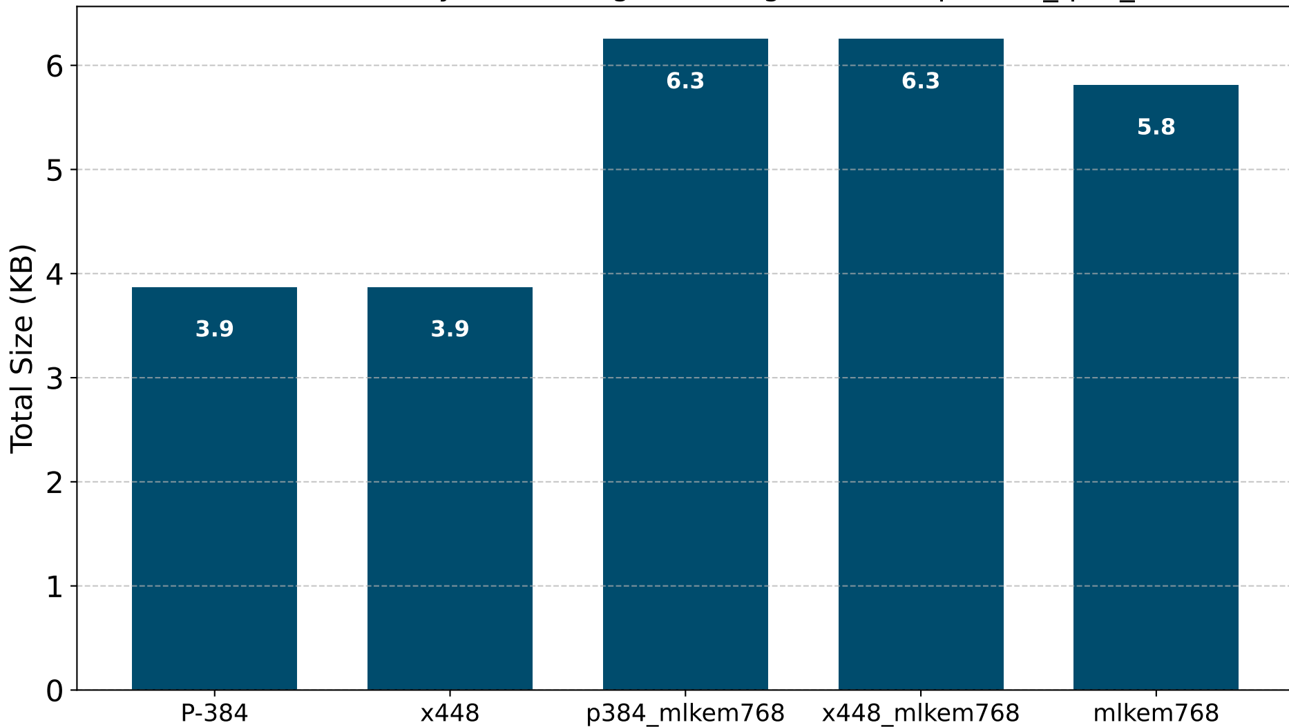
Total traffic size by KEM for signature algorithm secp384r1_quic_size
